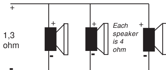
Three speakers in parallel
